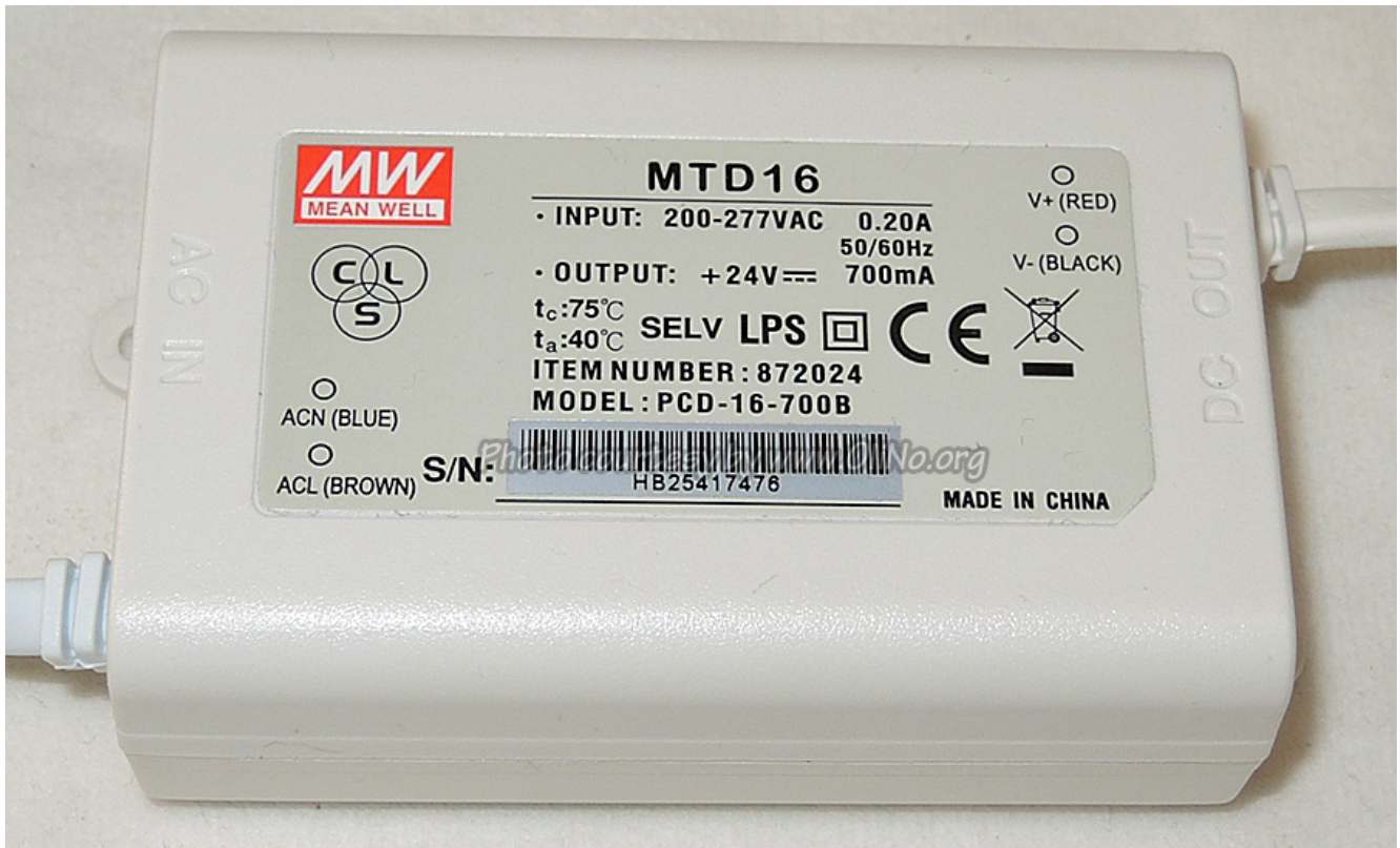
Power supply that was used.
