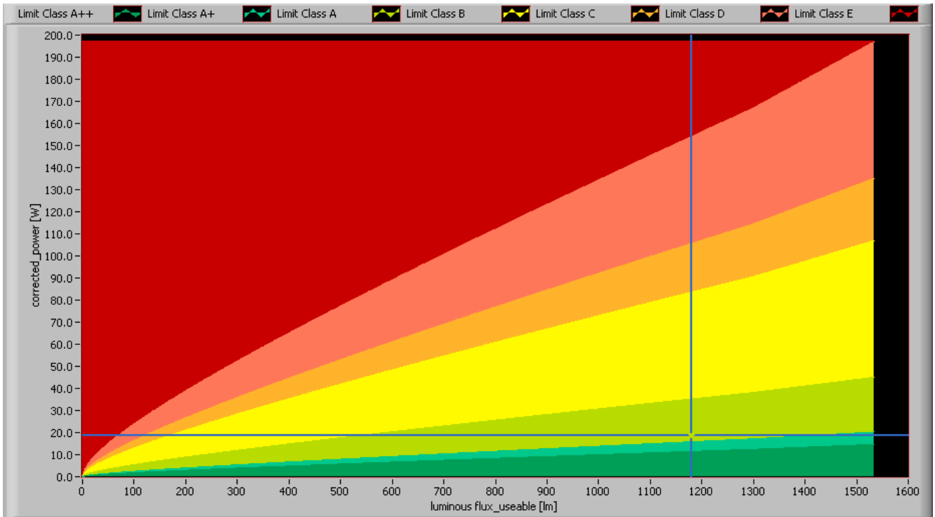
The lamp's performance in the lumen-Watt field, with the energy efficacy fields indicated.
