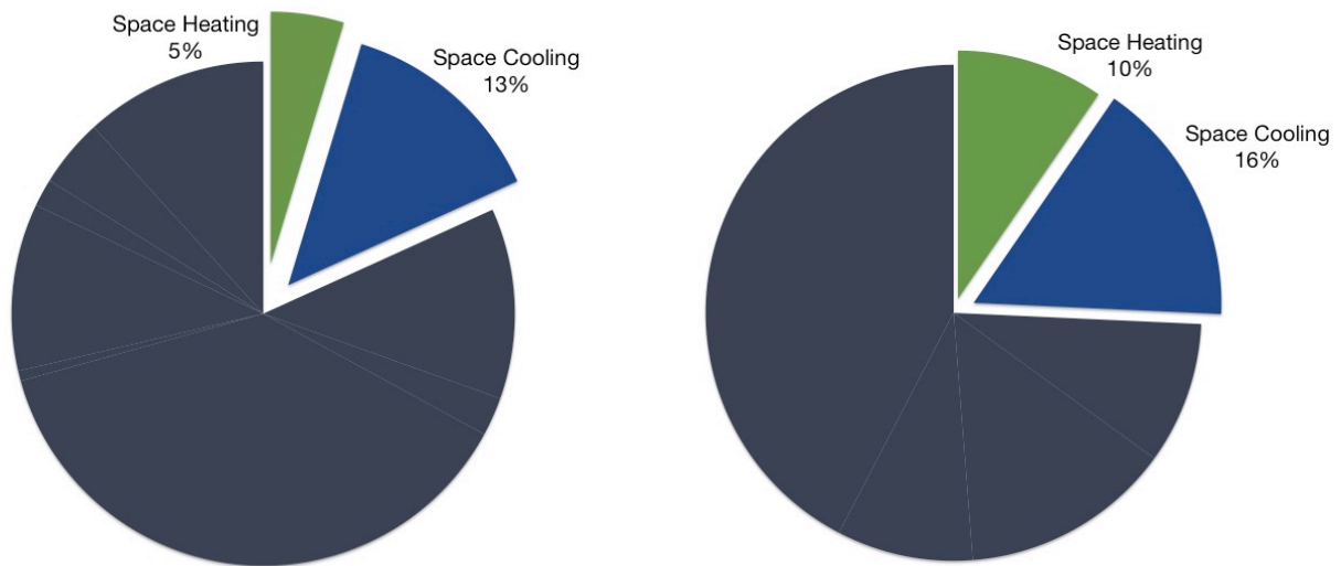
Figure 3: End-uses affected by Climate
