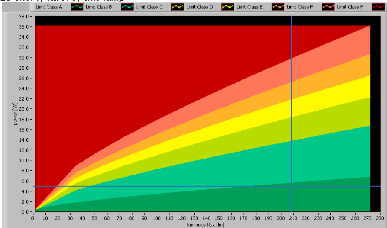
The lamp's performance in the lumen-Watt field, with the energy efficacy fields
