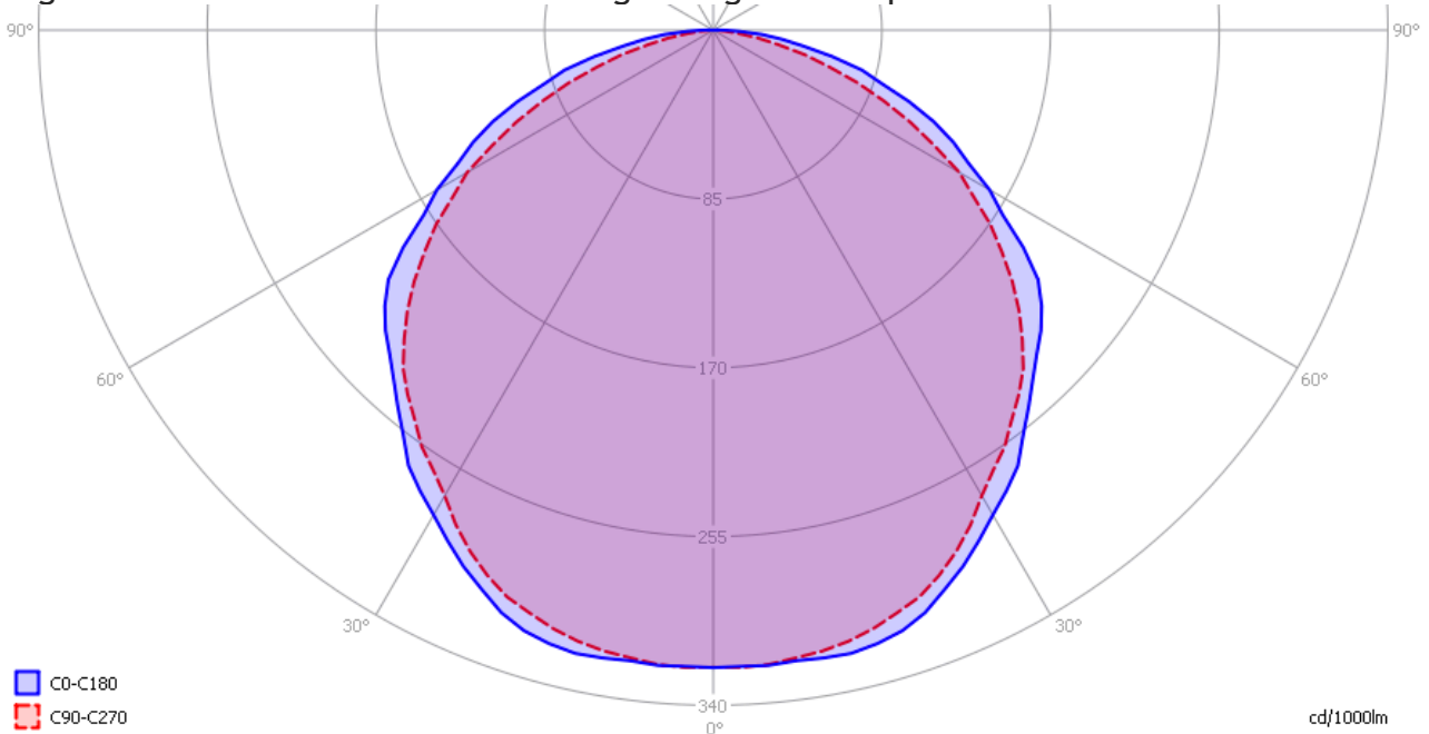
The light diagram giving the radiation pattern.
