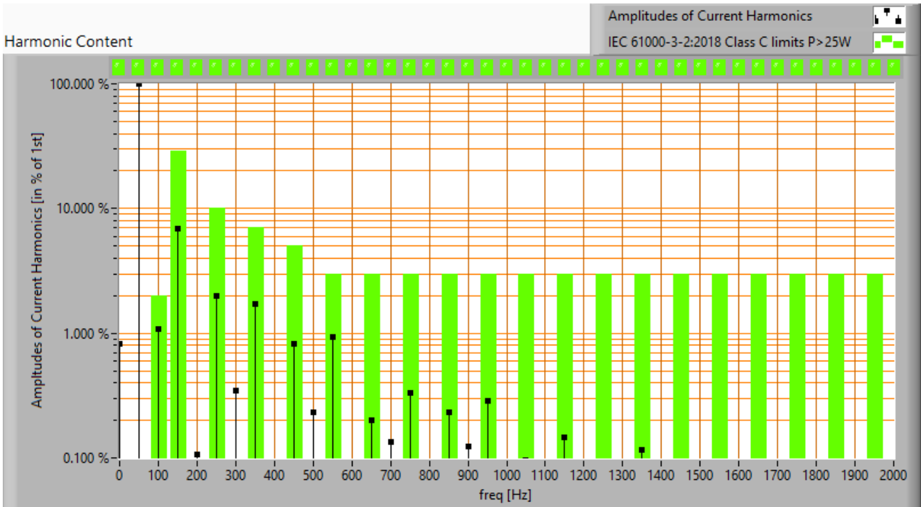
The harmonics in the current compared to the requirements in IEC61000-3-2:2018
