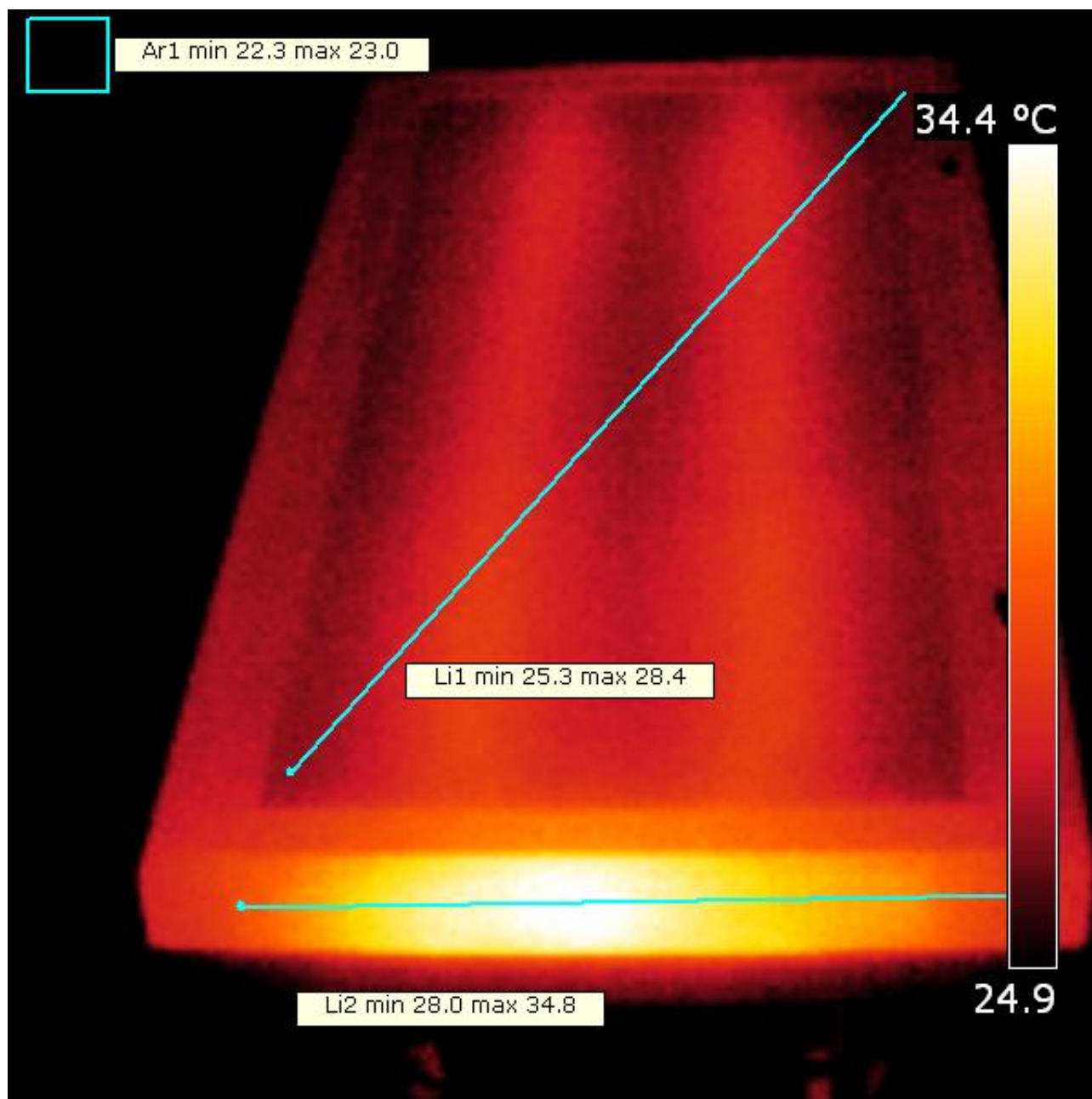
Temperature image. Close to the position of the power supply.
