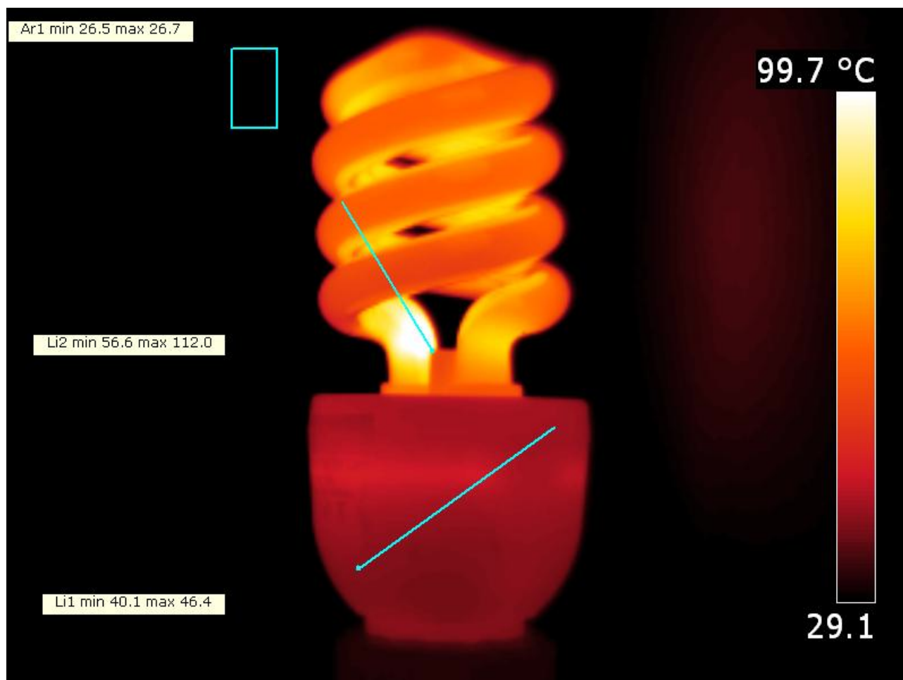
Temperature image of the lamp.
