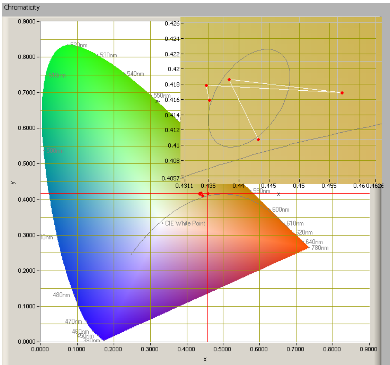
Color points of the 5 lamps in a 4-step MCAdams ellips.
