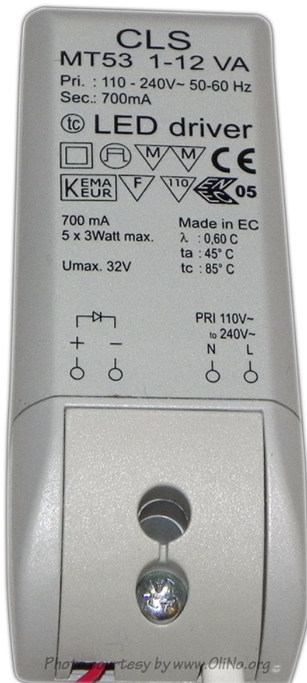
The used power supply.
