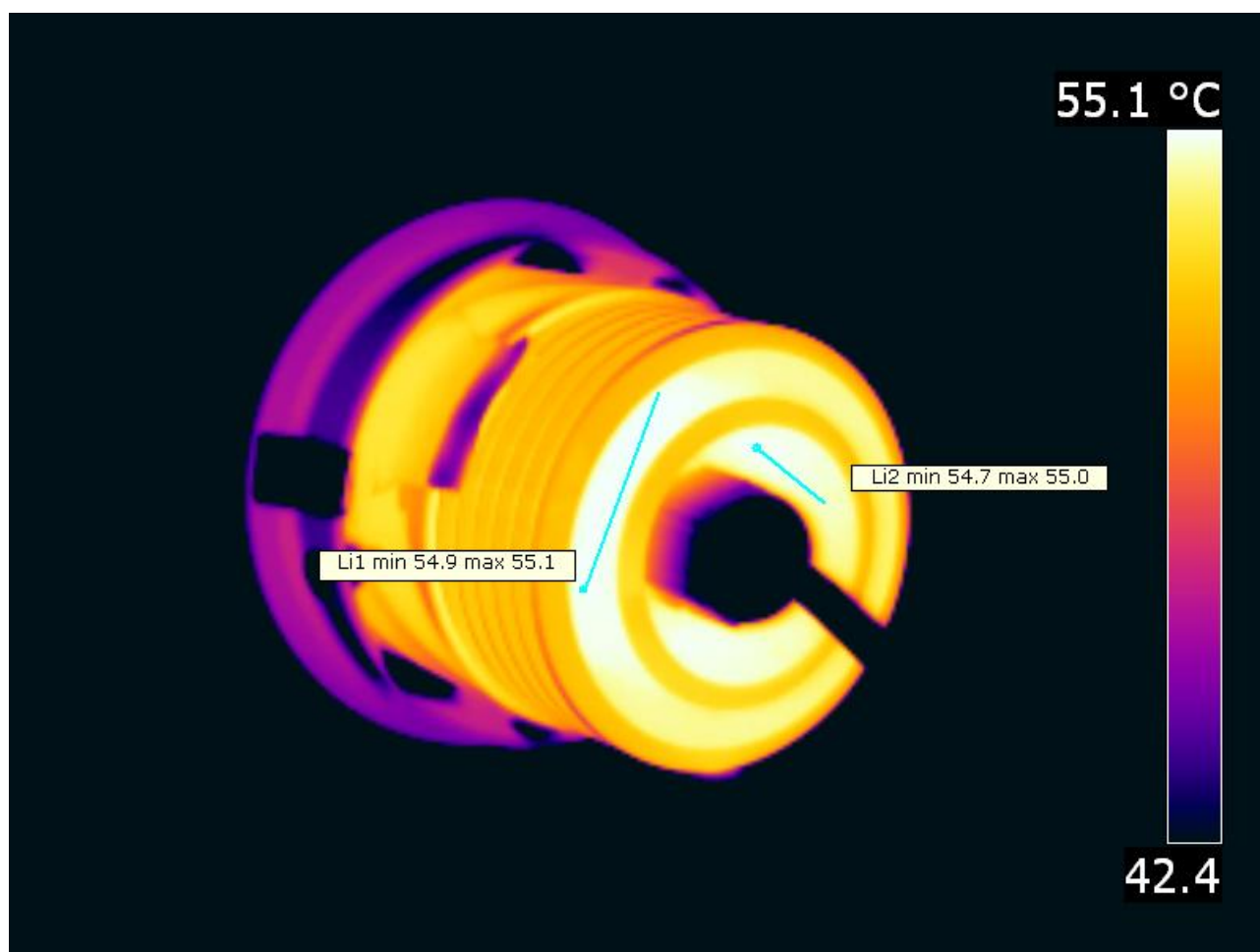
Temperature measurement of the back side.
