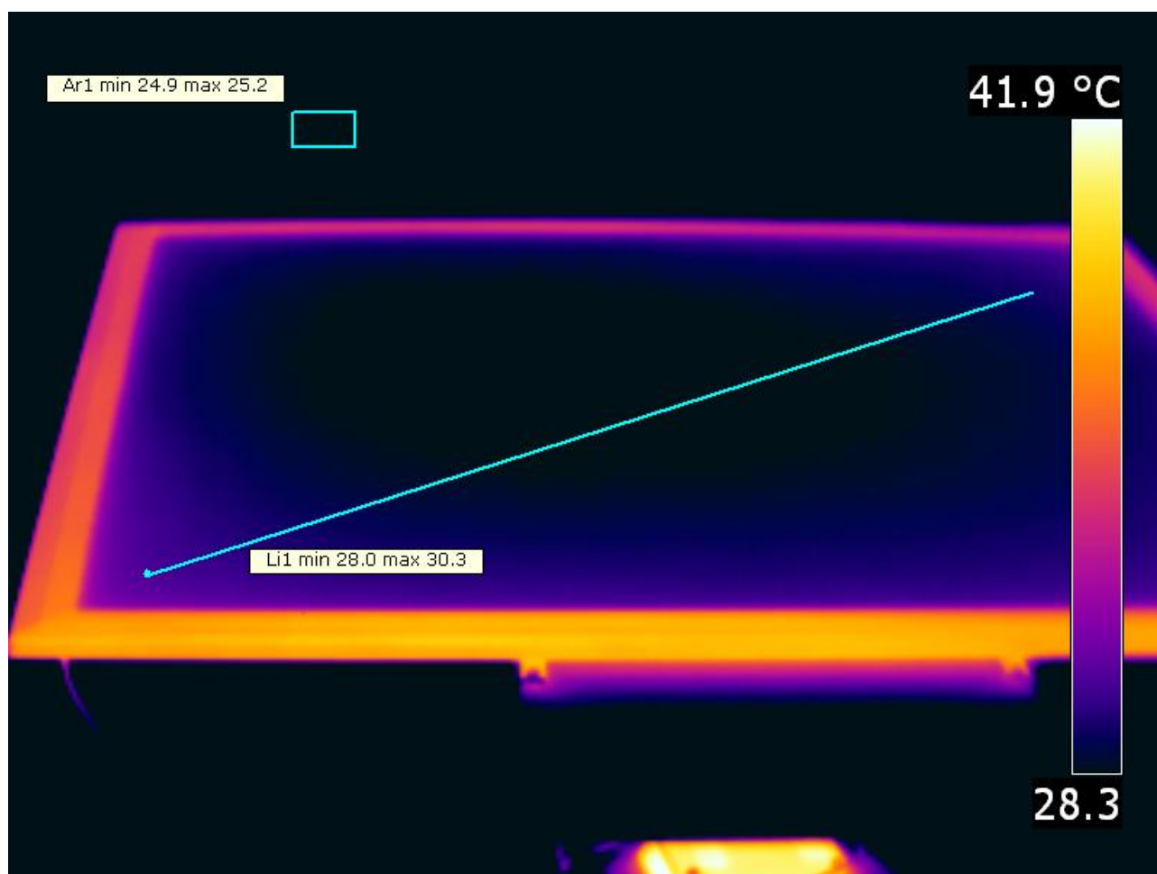
Temperature image of the panel.
