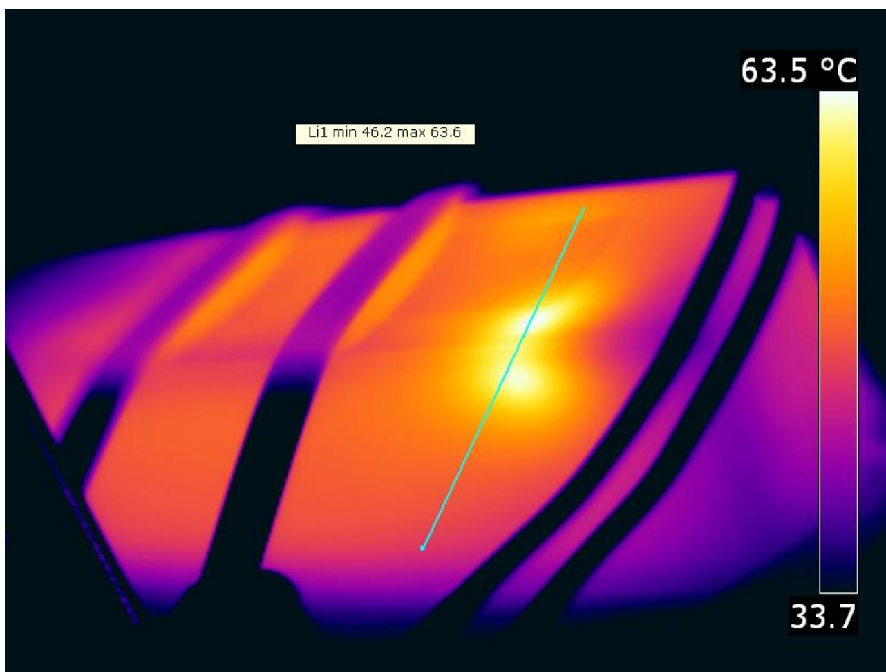
Temperature images. First the lamp and then the power supply.
