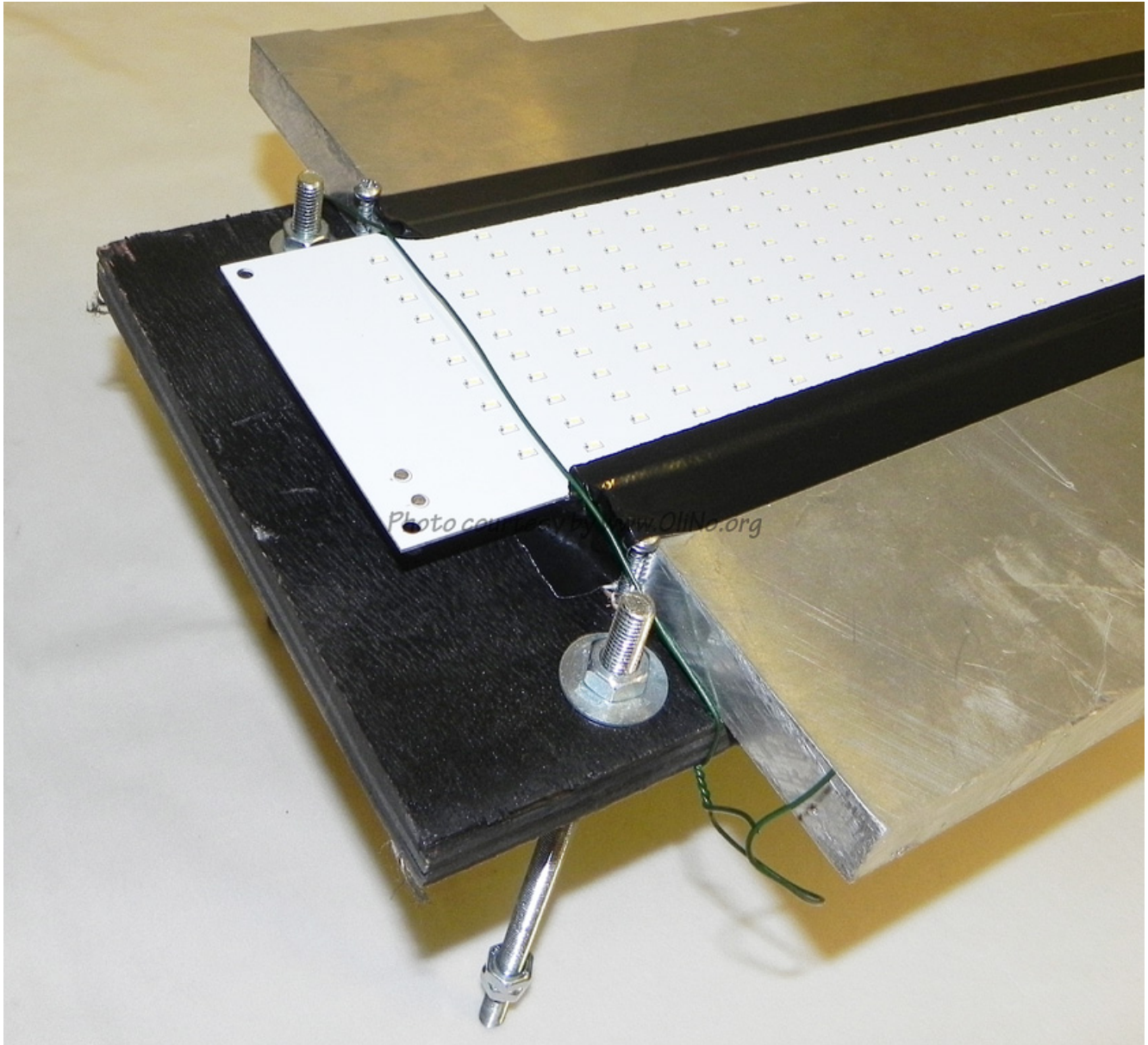
Plate mounted on a thick plate of aluminum for additional cooling.
